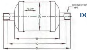
DCH DRIER WITH SAE CONNECTION DIMENSIONS DRAWING 1
