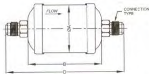
DCH DRIER WITH SAE CONNECTION DIMENSIONS DRAWING 1
